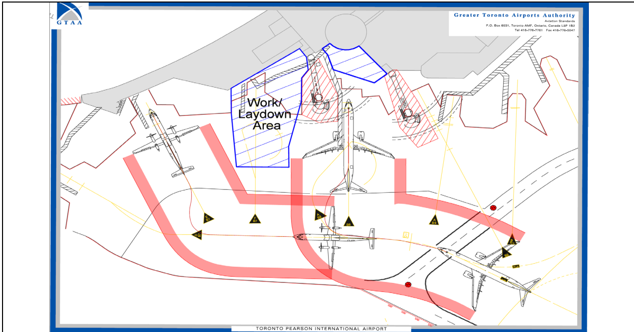
Figure 1 – Site Layout and Aircraft Clearances
