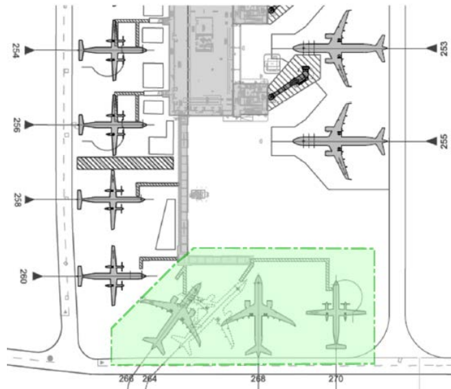
Figure 1 – Gate Closures (264, 266, 268, 270)
