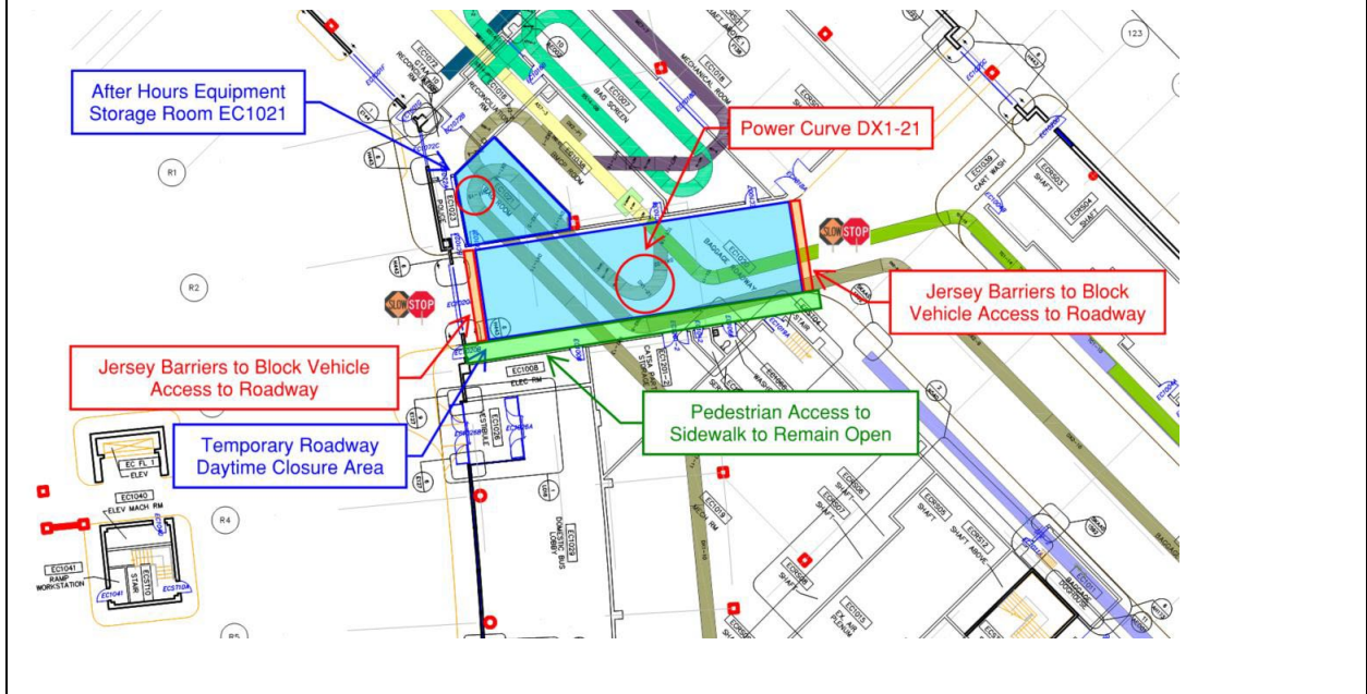
Figure 1 – Power Curve DX1 located above the ceiling of tunnel located near Stand 120.
